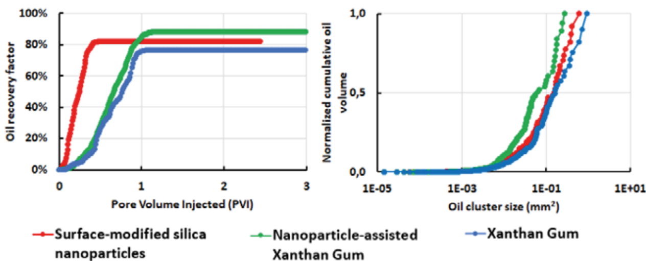
Figure 2: Left: oil recovery factor as a function of pore volume injected (PVI). Right: normalized cumulative residual oil volume as a function of oil cluster size. (Rueda et al., 2020)
