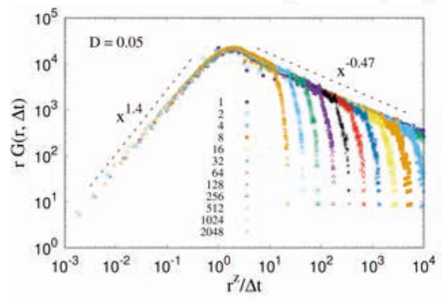
Figure 2. Pair correlation function G(r,\Delta t) for different values of \Delta t as indicated in the figure. The function shows two limiting power-law scaling for short and long time limits. The peak at r^{d_f}=\Delta t implies the most probable growth of the crack happens around r_t \sim \Delta t^{1/d_f} .
