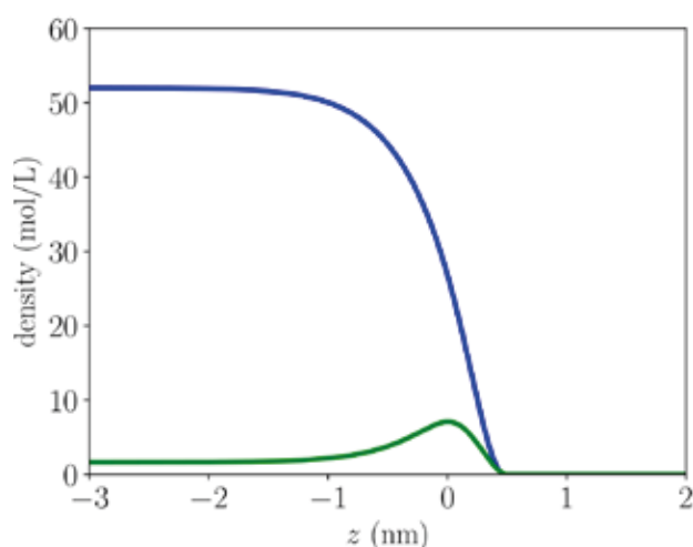
Fig. 1: Density profiles through a planar vapor—liquid interface for a binary mixture of water (blue) and 1-propanol (green) at 260 K. The accumulation of propanol in the surface is typical of surface-active mixtures. Here, z is the spatial position through the interface.
