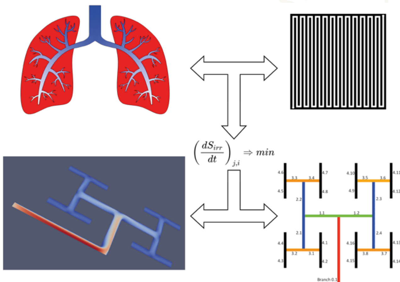
Figure 1. Taking inspiration from biological flow systems like the human lung (top left), conventional flow field plate patterns (top right) in polymer electrolyte fuel cells can be improved. This can be done by creating a tree-shaped pattern (bottom right) which can be further optimized by minimizing its entropy production. The advantage of this type of flow field pattern is that it delivers the gases in a uniform way (bottom left).
