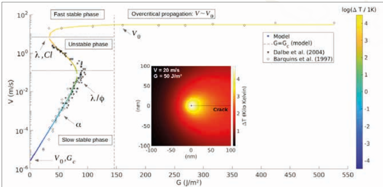
Fig. 1: Characteristic curve of energy release rate versus propagation velocity ( G, v ) theoretically obtained and fitted to experimental data (points) on fracture in tape glue, during tape peeling experiments. The unstable branch corresponds to G(v) decreasing, its presence is associated to a stick-slip instability. The tip temperature is visible in the colour bar. The arrows indicate which model parameters control the different parts of the curve. The inset shows the modelled temperature field around the crack tip, at the onset of the instability, v=20 m/s. After Vincent-Dospital et al., 2020a.
