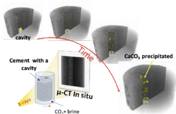
Figure 1. Perspective sketch of the home laboratory \mu -CT study. Selected \mu -CT images with cutaway-view highlight the calcium carbonate deposition inside the channel in the cement sample.
