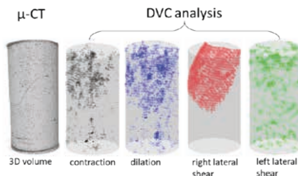
Figure 2. Results of in situ \mu -CT measurements using the HADES deformation rig, performed at the beamline ID19 at ESRF. The 3D reconstructed volume of shale at an axial pressure of 60 MPa and the corresponding incremental strain field obtained from DVC calculations are shown.
