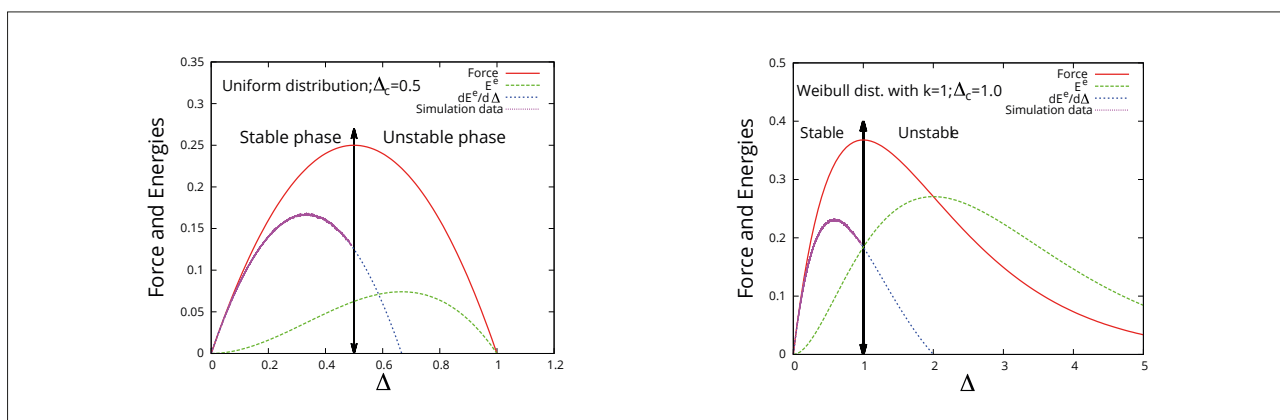
Fig. 2. Force, elastic energy and elastic energy variation vs. stretch for uniform and Weibull distribution of fiber strength. Results from simulations (purple) overlap with theoretically predicted curves (blue).
