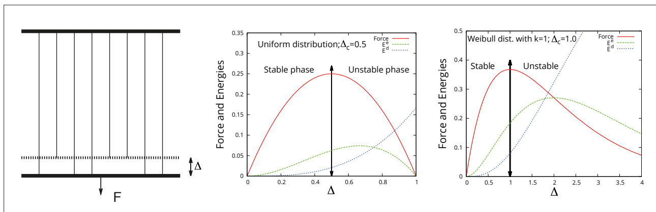
Fig. 1. The fiber bundle model and the force, elastic energy ( E^e ) and damage energy ( E^d ) vs. stretch for uniform and Weibull distribution of fiber strength.
