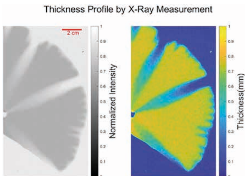
Figure 1. (Left) X-ray image of dissolved plaster sample captured by X-ray thickness gauge REX-CELL 4X from Flow Capture. The gray-scaled picture shown in the left panel is the normalized intensity of the X-ray measurement together with the color bar. (Right) Thickness profile of the dissolved plaster sample is displayed with the gradient-color picture together with the color bar.
