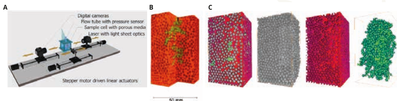
Fig. 2. A The scanner is based on optical index matching and fluorescence. A random packing of 3 mm glass beads forms the porous medium, index matched with two immiscible fluids. The fluids contain different fluorescent dyes that are excited with a 2D laser sheet, that is driven through the sample during a scan. The fluid phases appear on the images with different colors, making them distinguishable through the analysis. B Raw 3D data. The 2D images captured as frames by the cameras are put together to build up the third dimension. C Segmented phases. The porous medium and the two liquid phases are fully separated.
